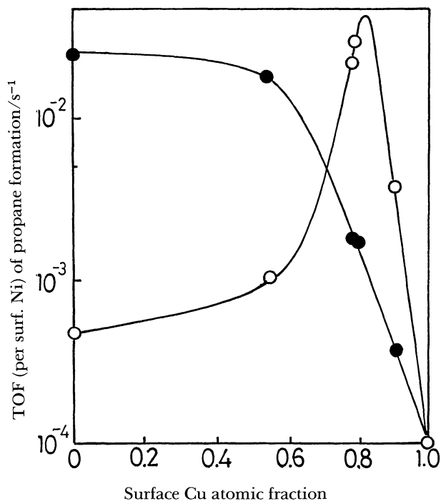
Fig. 8. Dependence of TOF of propane formation at 200 K upon the surface Cu atomic fraction.
