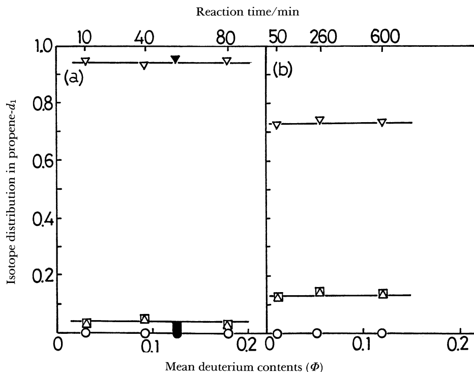
Fig. 6. Time course of the isotopic distribution in monodeuteriopropene during C_3H_6 - D_2 reaction over (a) Ni metal at 200 K, and (b) Cu metal at 263 K. p_{D_2}=6.7 kPa, p_{C_3H_6}=2.0 kPa, Catalyst=1 g. Open symbols: over D-surfaces, closed symbols: over E-surfaces. \square : c -1- d_1 , \triangle : t -1- d_1 , \nabla : 2- d_1 , \circ : 3- d_1 .
