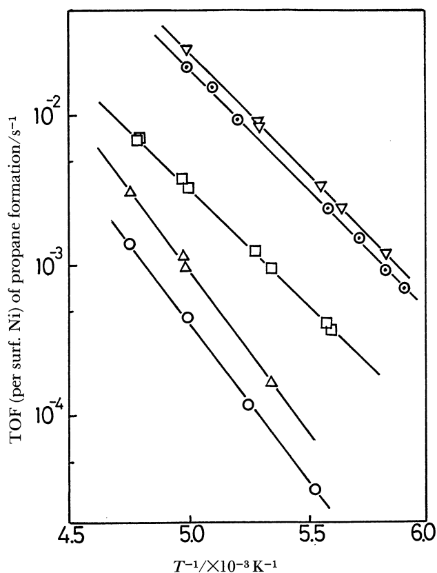
Fig. 2. Temperature dependence of TOF of propane formation (D-surface) over various catalysts. p_{D_2}=6.7 \text{ kPa} , p_{C_3H_6}=2.0 \text{ kPa} , Catalyst=1 g. \circ : Ni, \Delta : Ni-Cu(0.5), \odot : Ni-Cu(25), \nabla : Ni-Cu(60), \square : Ni-Cu(90).
