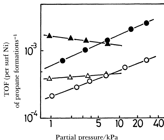
Fig. 3. Pressure dependence of TOF of propane formation (D-surface) over (a) Ni metal at 210 K (open symbols), and (b) Ni-Cu(25) alloy catalyst at 180 K (closed symbols). \circ : Dependence of H_2 partial pressure ( p_{C_3H_6}=3.3 \text{ kPa} , constant). \Delta : Dependence of C_3H_6 partial pressure ( p_{H_2}=6.7 \text{ kPa} , constant).
