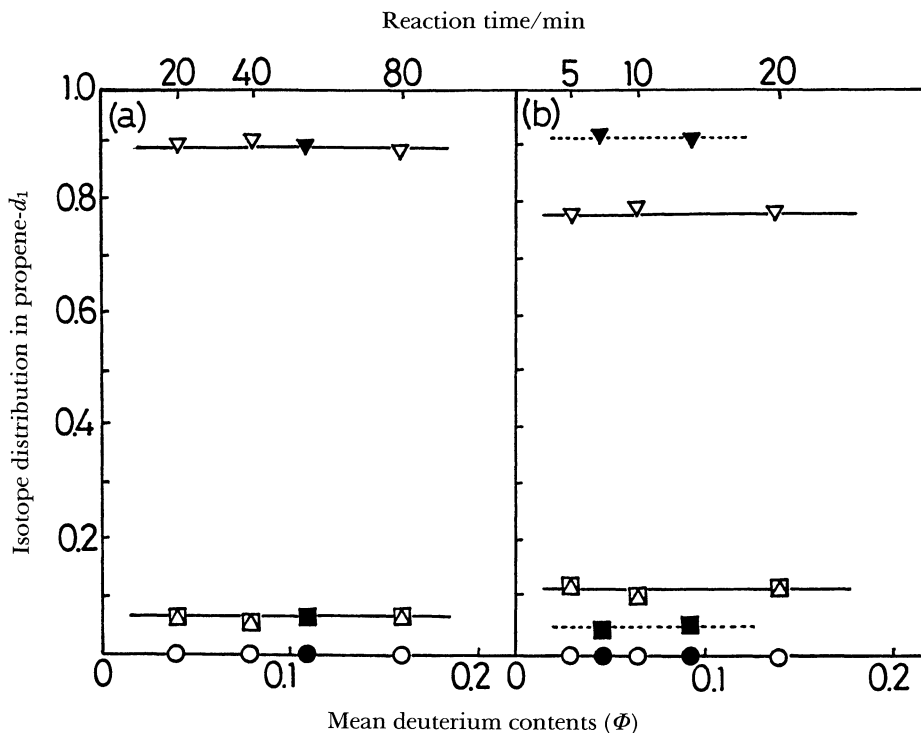
Fig. 7. Time course of the isotopic distribution of monodeuteriopropene during C_3H_6 - D_2 reaction over (a) Ni-Cu(0.5) alloy at 190 K, and (b) Ni-Cu(25) alloy at 180 K.
